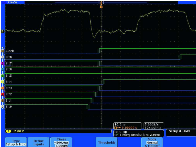
Multichannel setup and hold triggering highlighting multiple violations (MSO4000).
